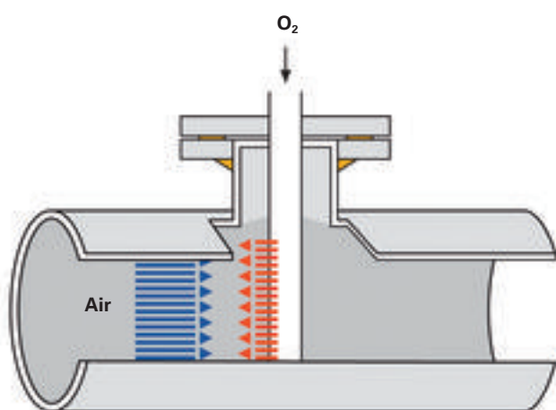
Oxygen mixer for combustion air enrichment
